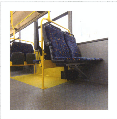
Low floor along the whole vehicle, seating fixed to the side walls
