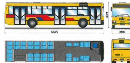
JELCZ M121M, M121MB
